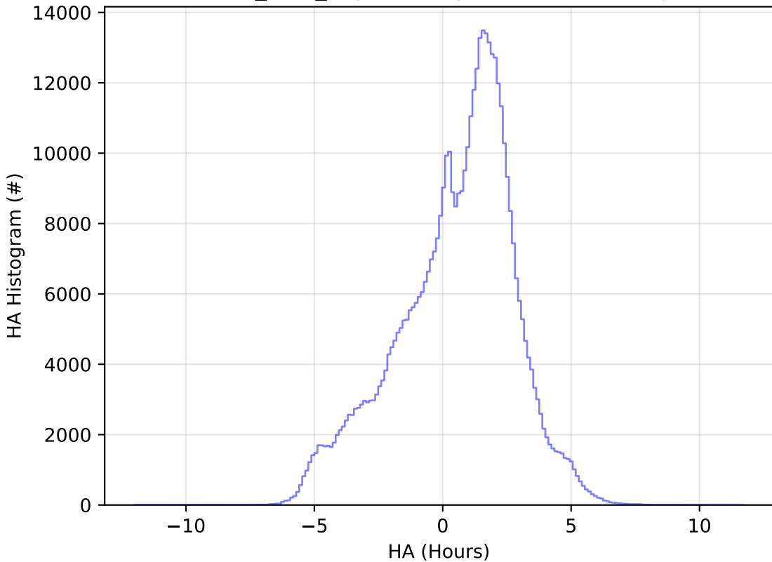
baseline_v3.5_10yrs All sky i band: HA Histogram
