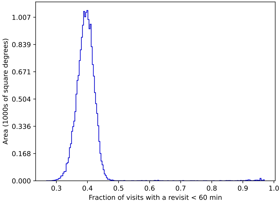
baseline_v3.5_10yrs gri WFD: Fraction of visits with a revisit < 60 min
