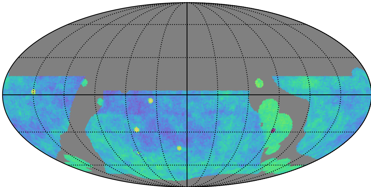
baseline_v3.5_10yrs gri WFD: Fraction of visits in pairs (20-90 min)
