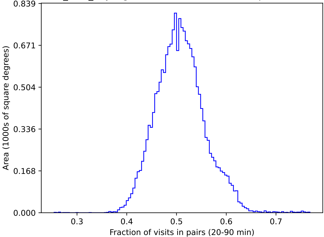
baseline_v3.5_10yrs gri WFD: Fraction of visits in pairs (20-90 min)
