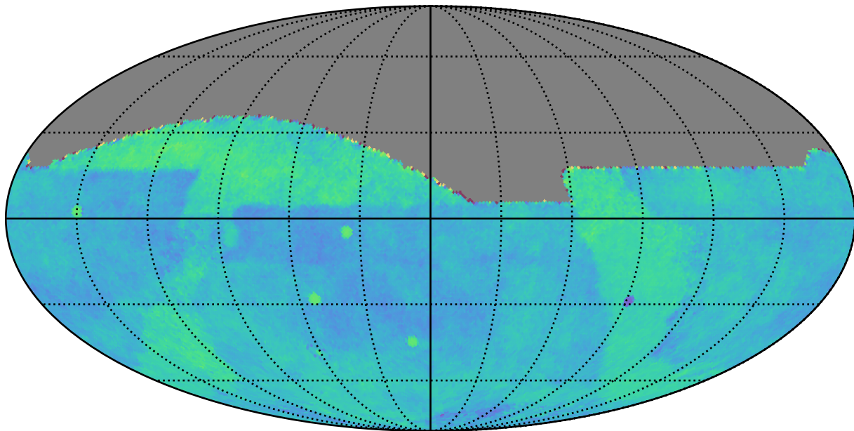
baseline_v3.5_10yrs gri All sky: Fraction of visits in pairs (20-90 min)
