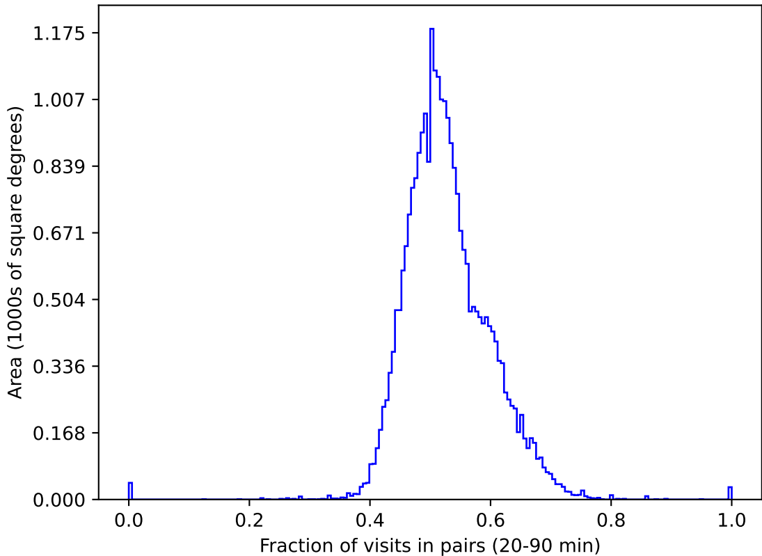
baseline_v3.5_10yrs gri All sky: Fraction of visits in pairs (20-90 min)
