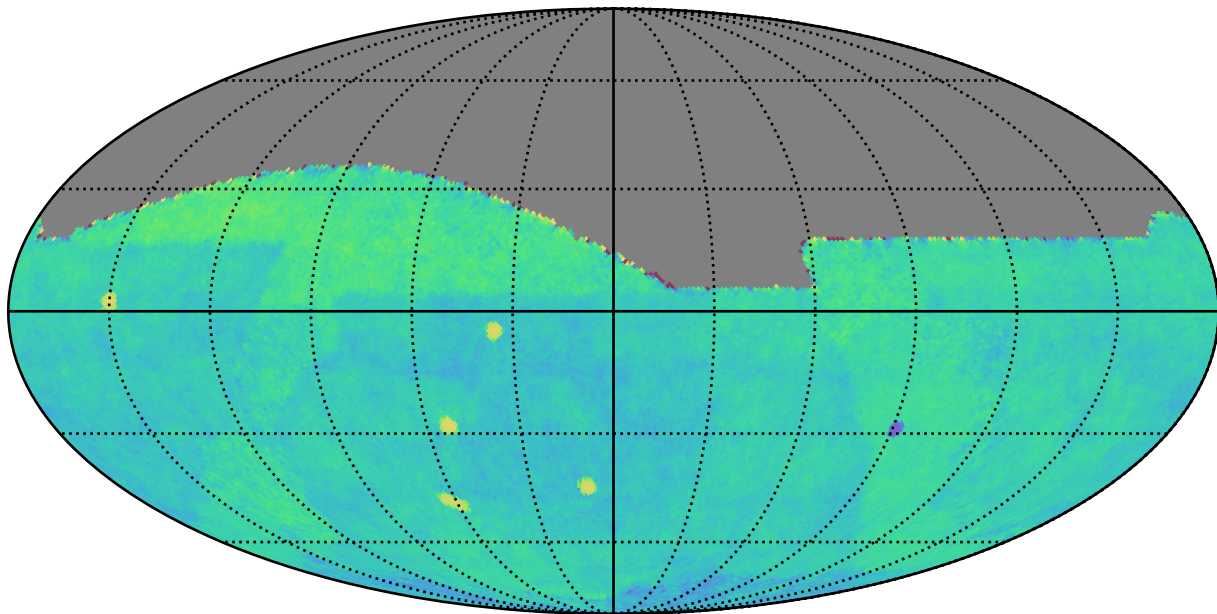
baseline_v3.5_10yrs gri All sky: Fraction of visits in pairs (10-60 min)
