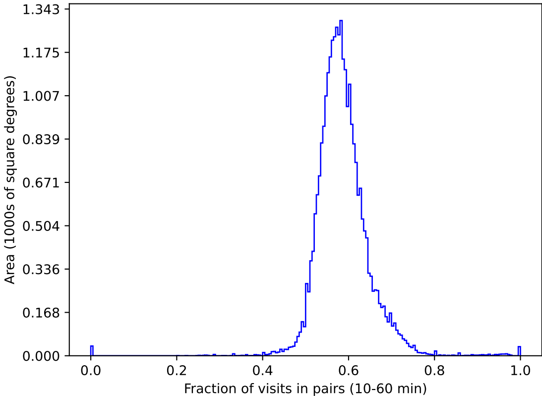
baseline_v3.5_10yrs gri All sky: Fraction of visits in pairs (10-60 min)
