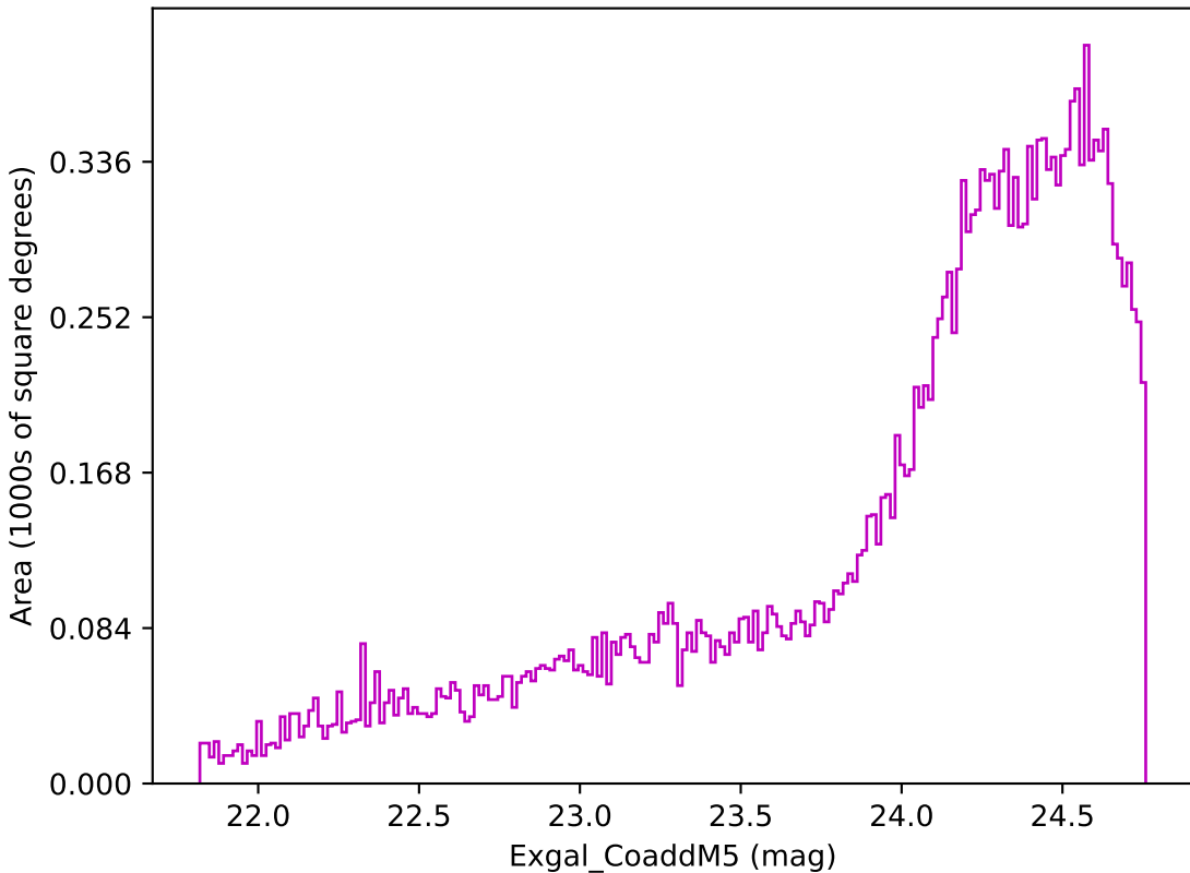
baseline_v3.5_10yrs Yr 3-4 z band: Exgal_CoaddM5
