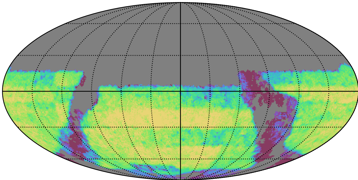
baseline_v3.5_10yrs Yr 3-4 y band: Exgal_CoaddM5
