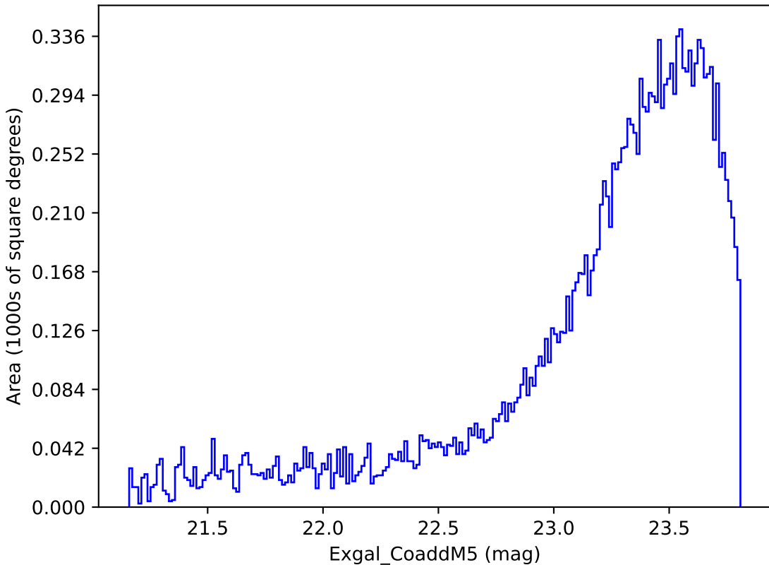
baseline_v3.5_10yrs Yr 3-4 y band: Exgal_CoaddM5
