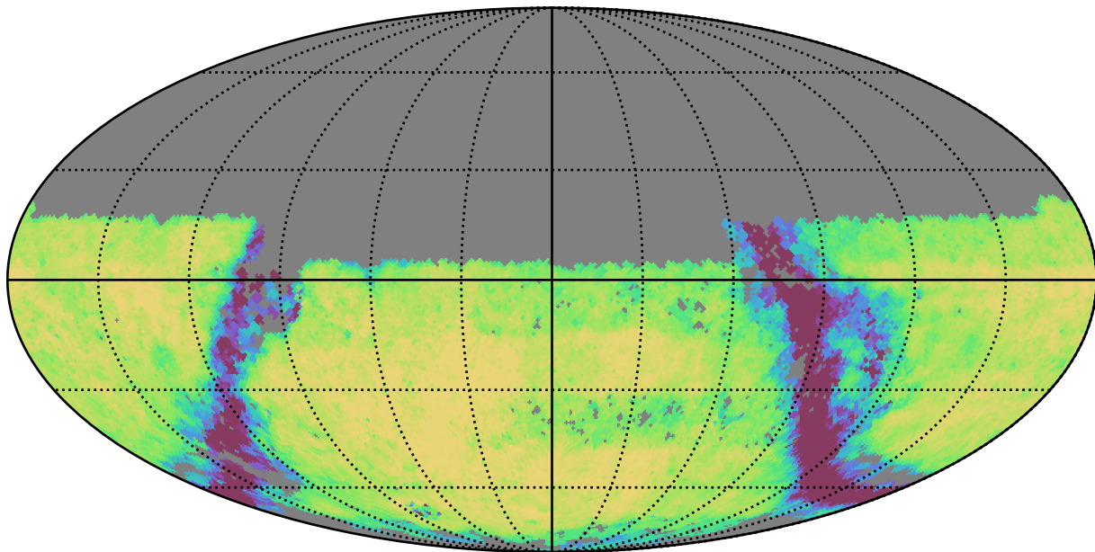
baseline_v3.5_10yrs Yr 3-4 u band: Exgal_CoaddM5
