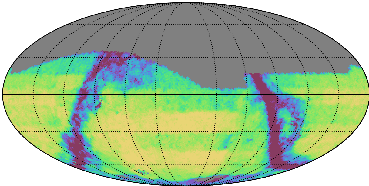
baseline_v3.5_10yrs Yr 3-4 r band: Exgal_CoaddM5
