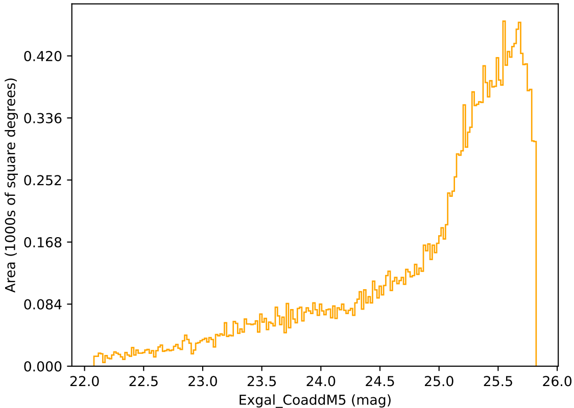
baseline_v3.5_10yrs Yr 3-4 r band: Exgal_CoaddM5
