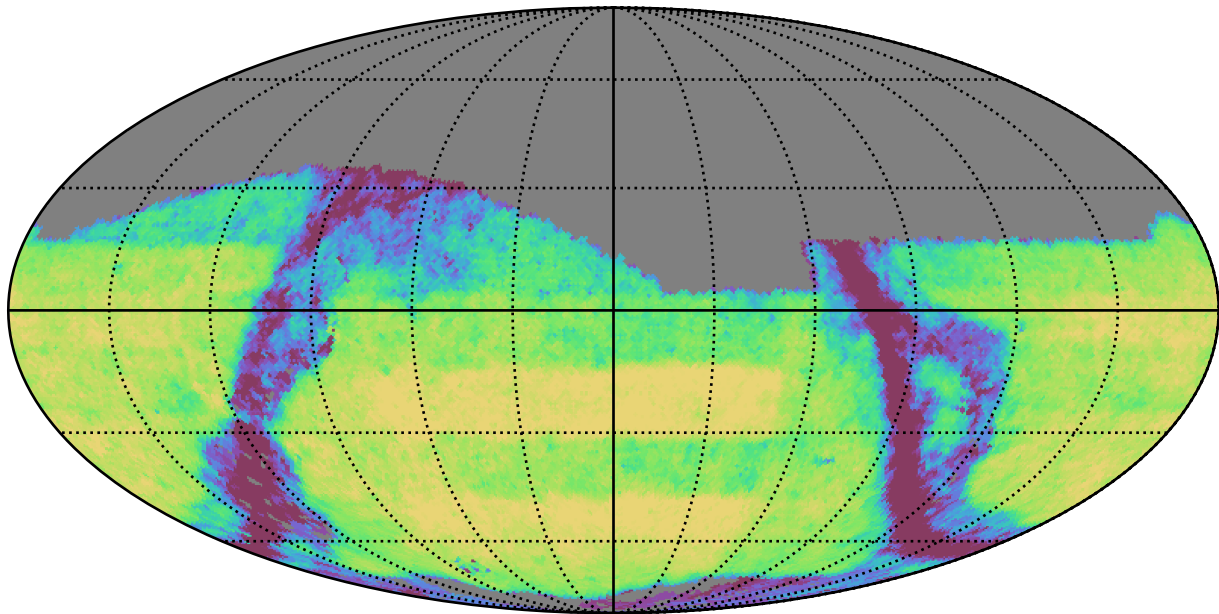
baseline_v3.5_10yrs Yr 3-4 i band: Exgal_CoaddM5
