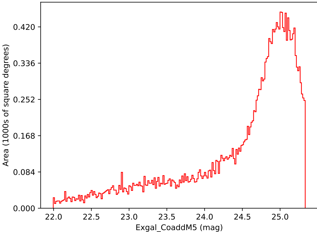
baseline_v3.5_10yrs Yr 3-4 i band: Exgal_CoaddM5
