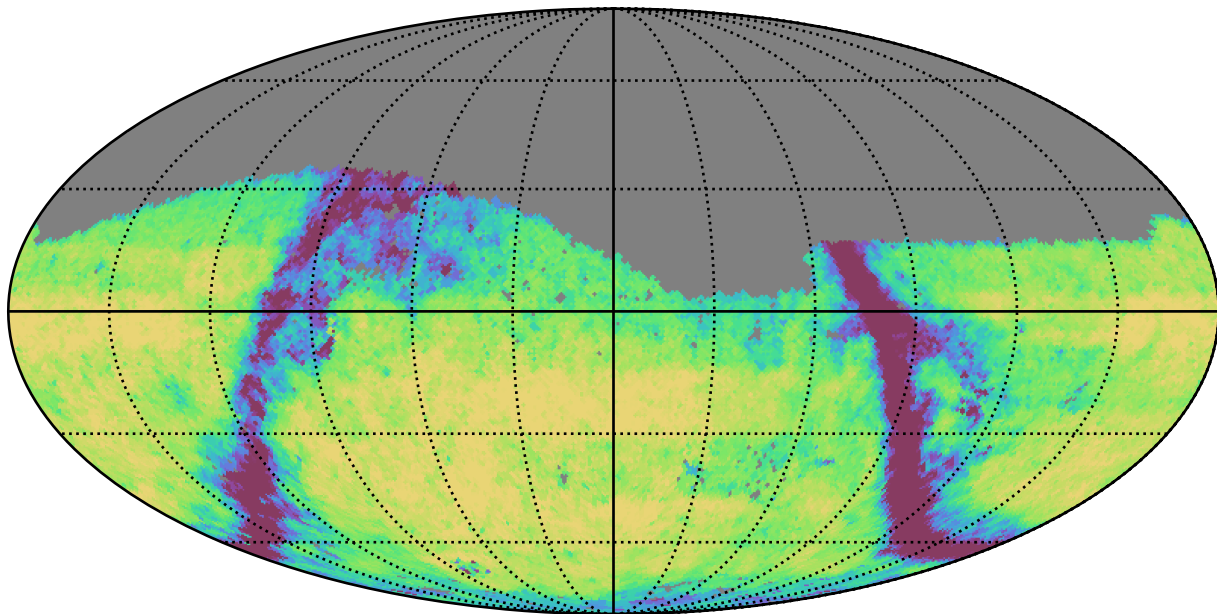
baseline_v3.5_10yrs Yr 3-4 g band: Exgal_CoaddM5
