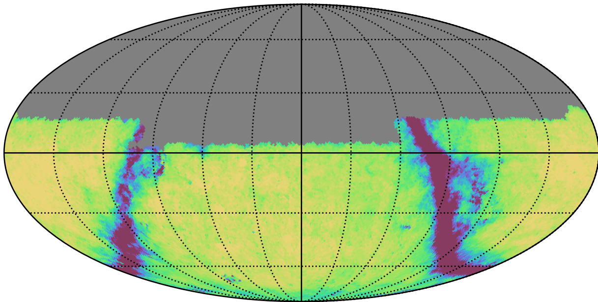
baseline_v3.5_10yrs Yr 1 u band: Exgal_CoaddM5
