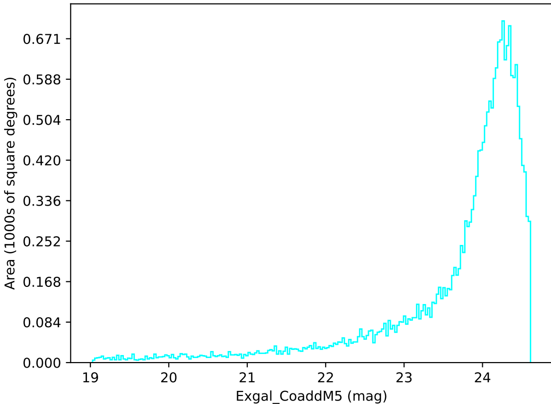
baseline_v3.5_10yrs Yr 1 u band: Exgal_CoaddM5
