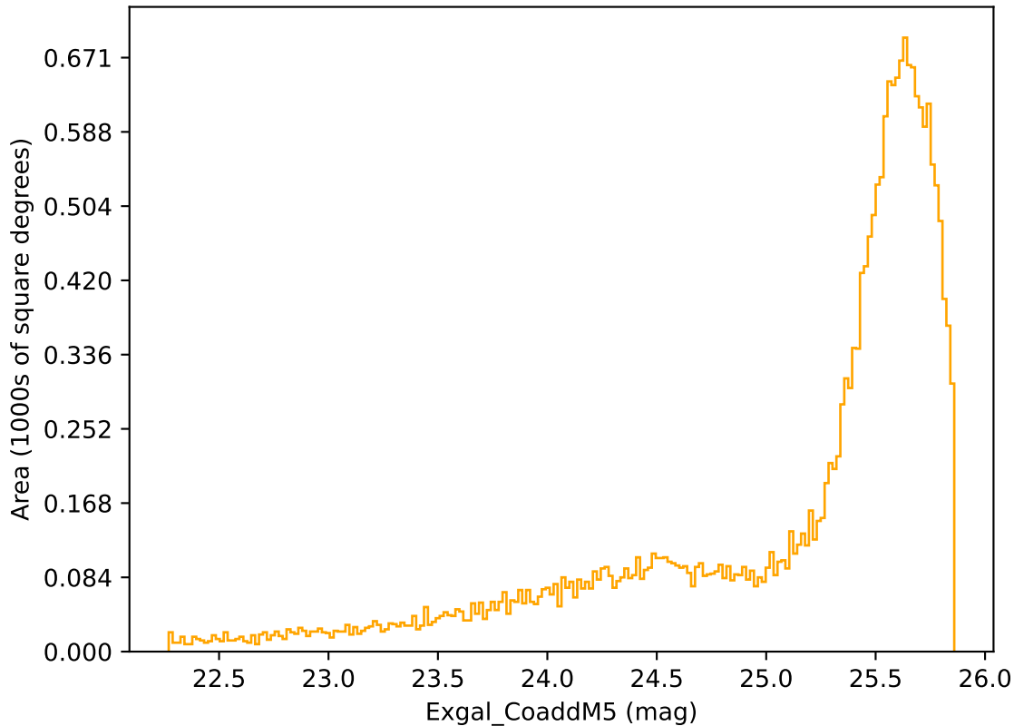
baseline_v3.5_10yrs Yr 1 r band: Exgal_CoaddM5
