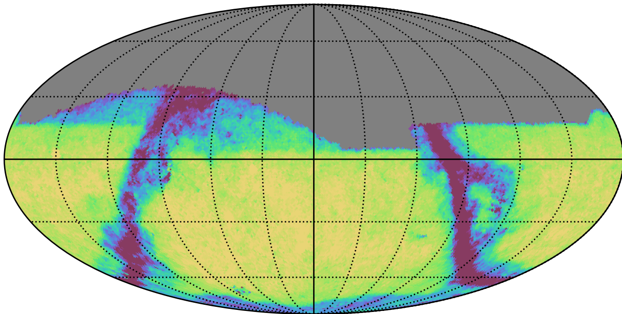
baseline_v3.5_10yrs Yr 1 i band: Exgal_CoaddM5
