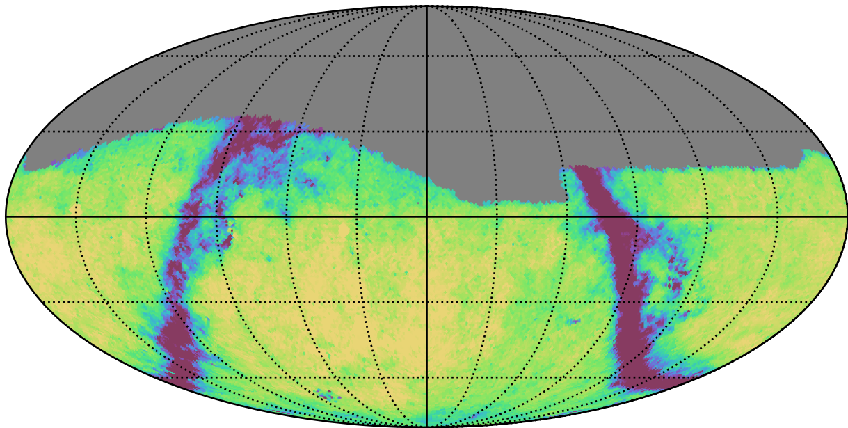
baseline_v3.5_10yrs Yr 1 g band: Exgal_CoaddM5
