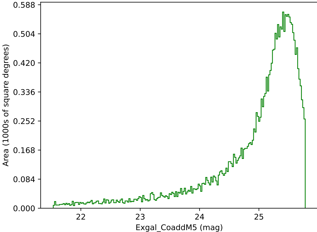
baseline_v3.5_10yrs Yr 1 g band: Exgal_CoaddM5
