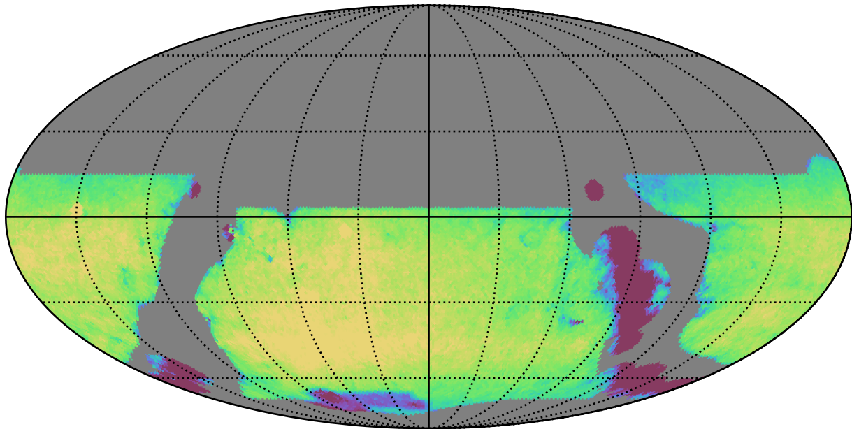
baseline_v3.5_10yrs WFD z band: Exgal_CoaddM5
