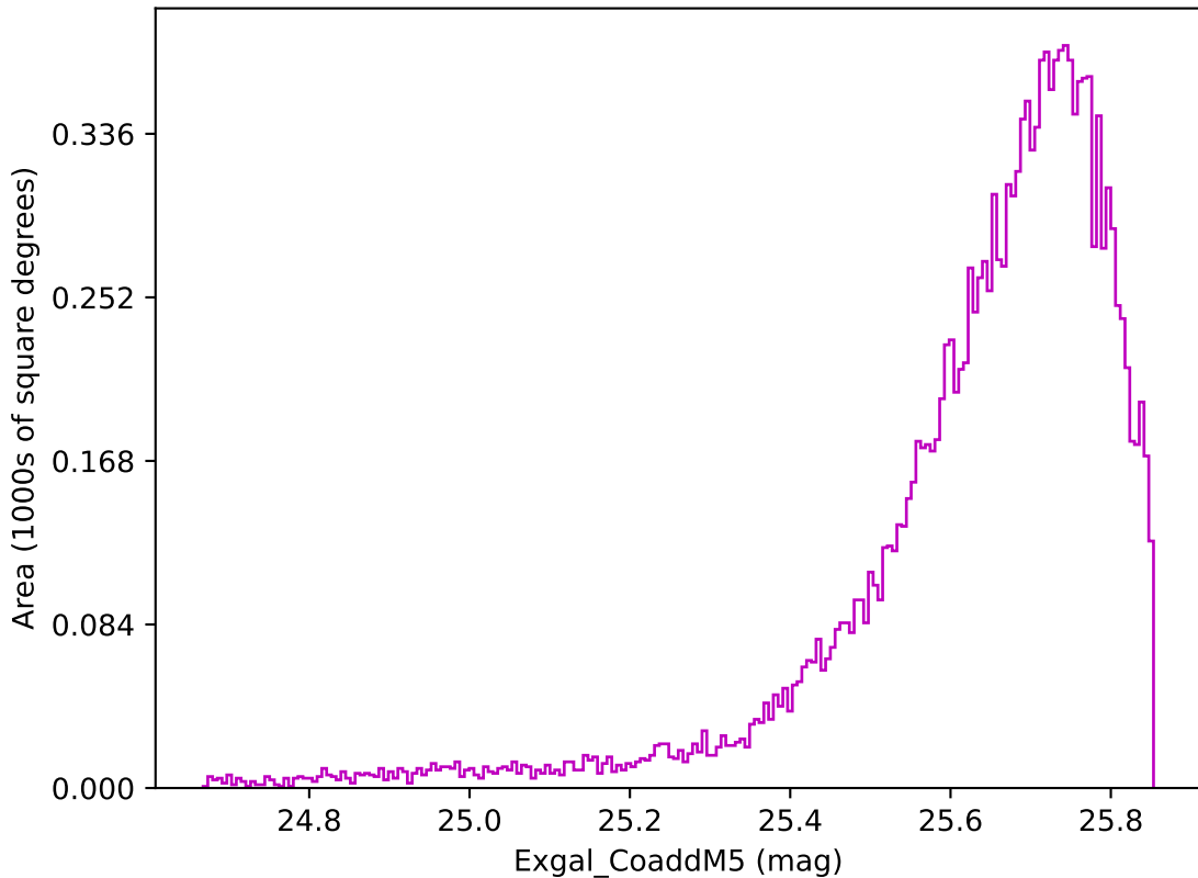
baseline_v3.5_10yrs WFD z band: Exgal_CoaddM5
