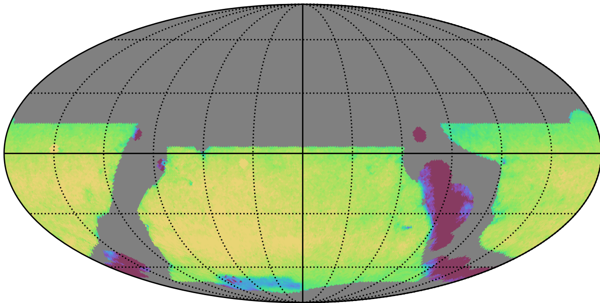
baseline_v3.5_10yrs WFD y band: Exgal_CoaddM5
