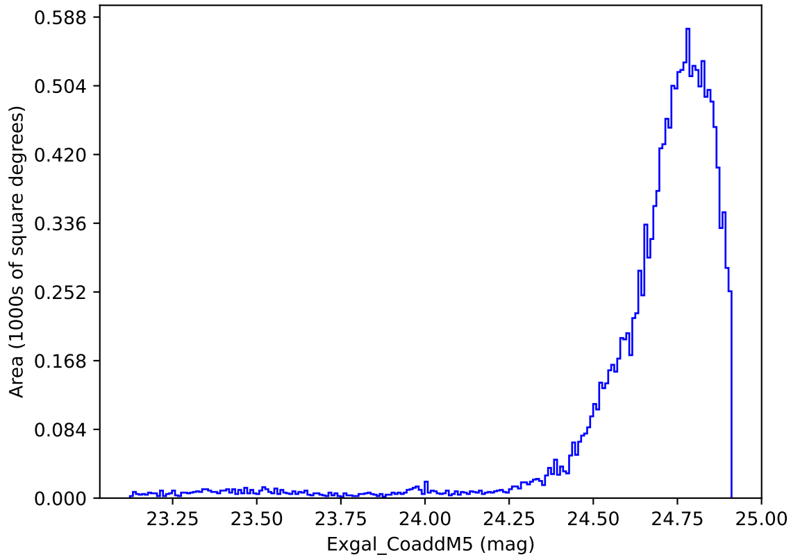
baseline_v3.5_10yrs WFD y band: Exgal_CoaddM5
