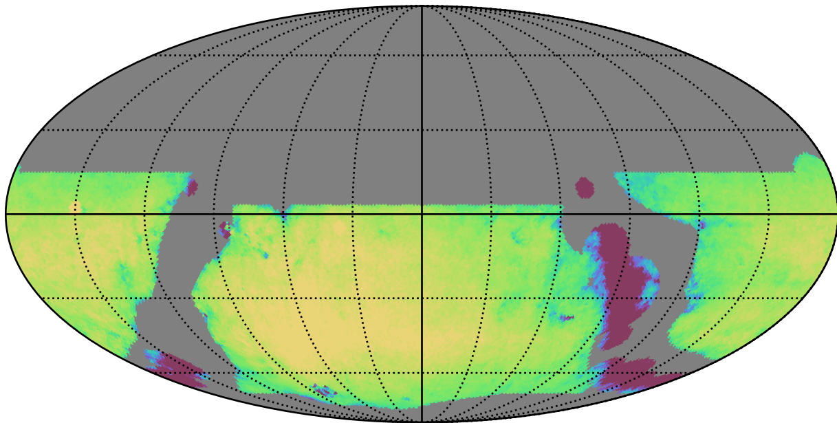
baseline_v3.5_10yrs WFD r band: Exgal_CoaddM5
