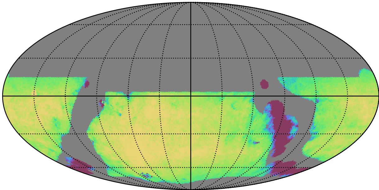
baseline_v3.5_10yrs WFD i band: Exgal_CoaddM5
