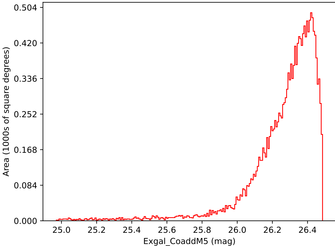
baseline_v3.5_10yrs WFD i band: Exgal_CoaddM5
