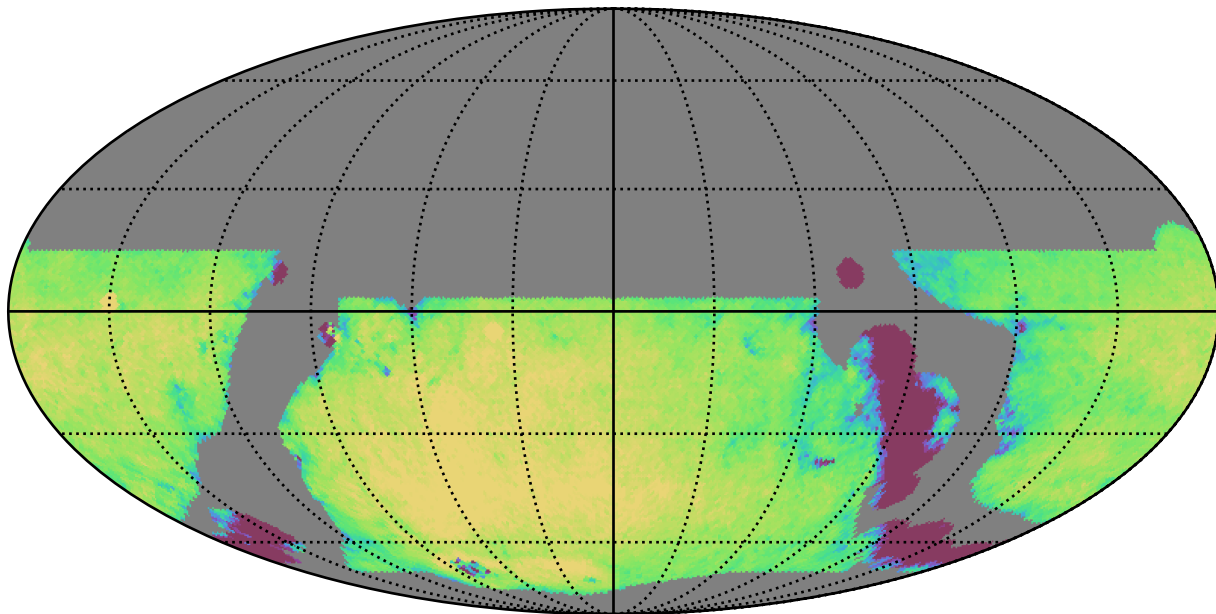
baseline_v3.5_10yrs WFD g band: Exgal_CoaddM5
