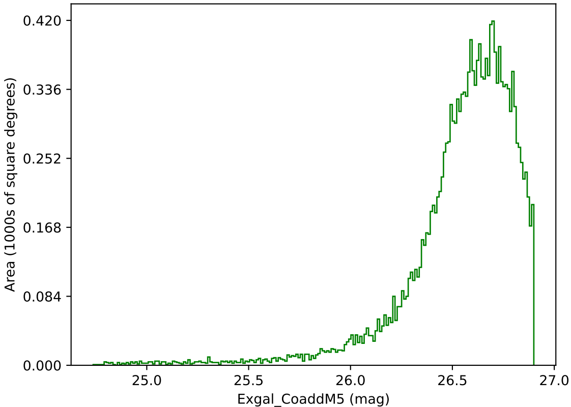
baseline_v3.5_10yrs WFD g band: Exgal_CoaddM5
