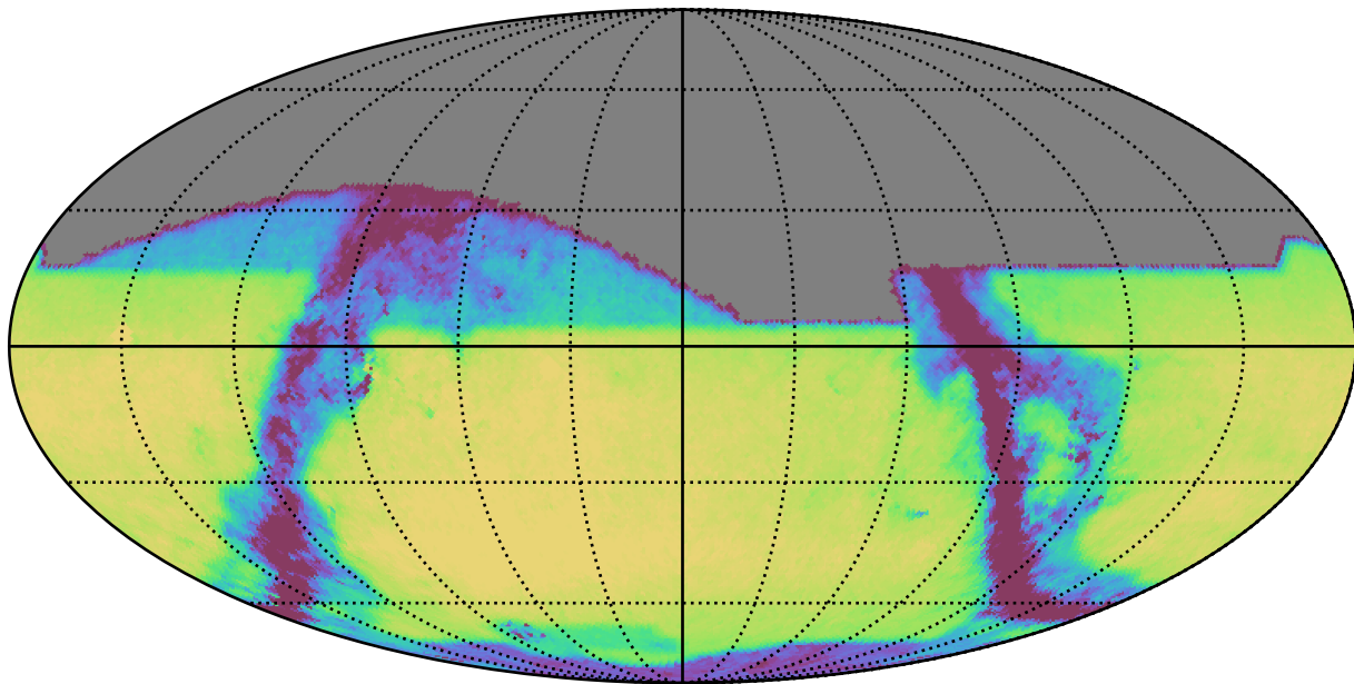
baseline_v3.5_10yrs All sky z band: Exgal_CoaddM5
