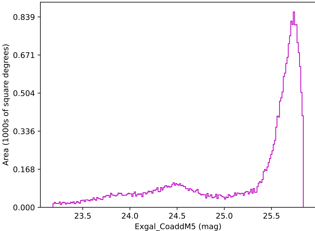
baseline_v3.5_10yrs All sky z band: Exgal_CoaddM5
