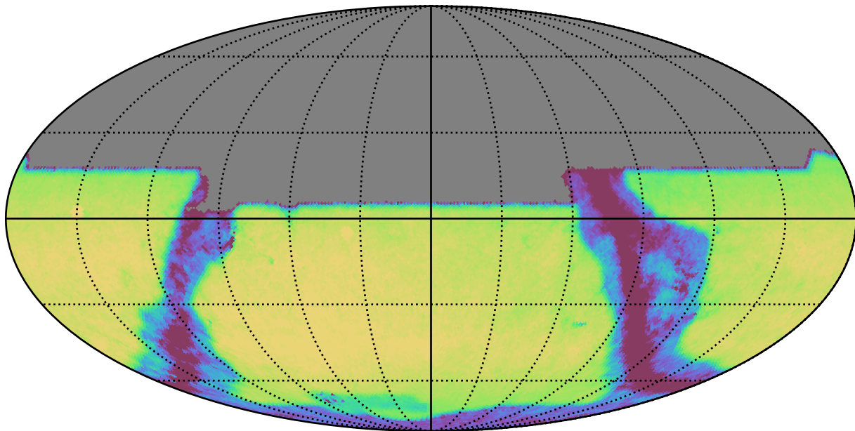
baseline_v3.5_10yrs All sky y band: Exgal_CoaddM5
