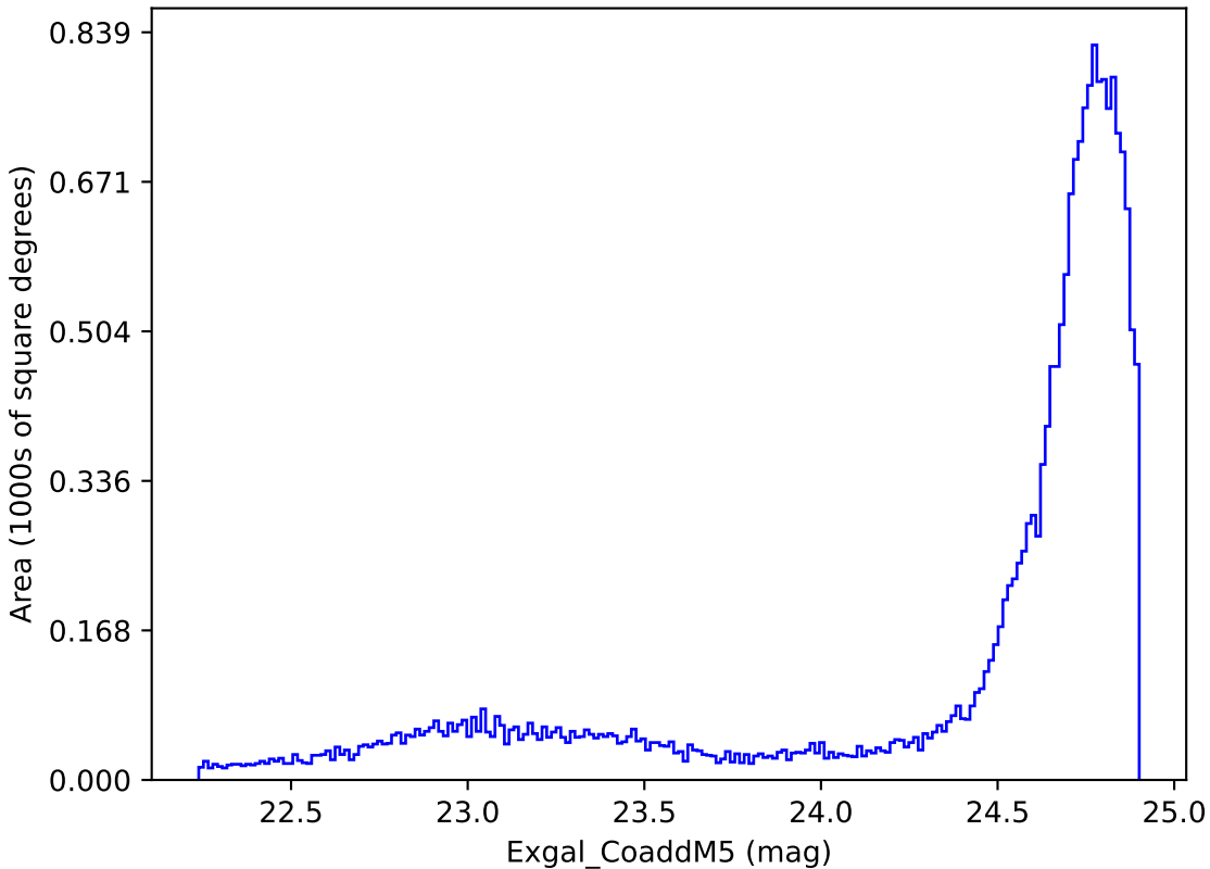
baseline_v3.5_10yrs All sky y band: Exgal_CoaddM5
