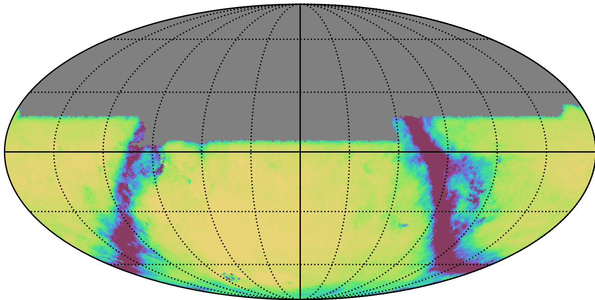
baseline_v3.5_10yrs All sky u band: Exgal_CoaddM5
