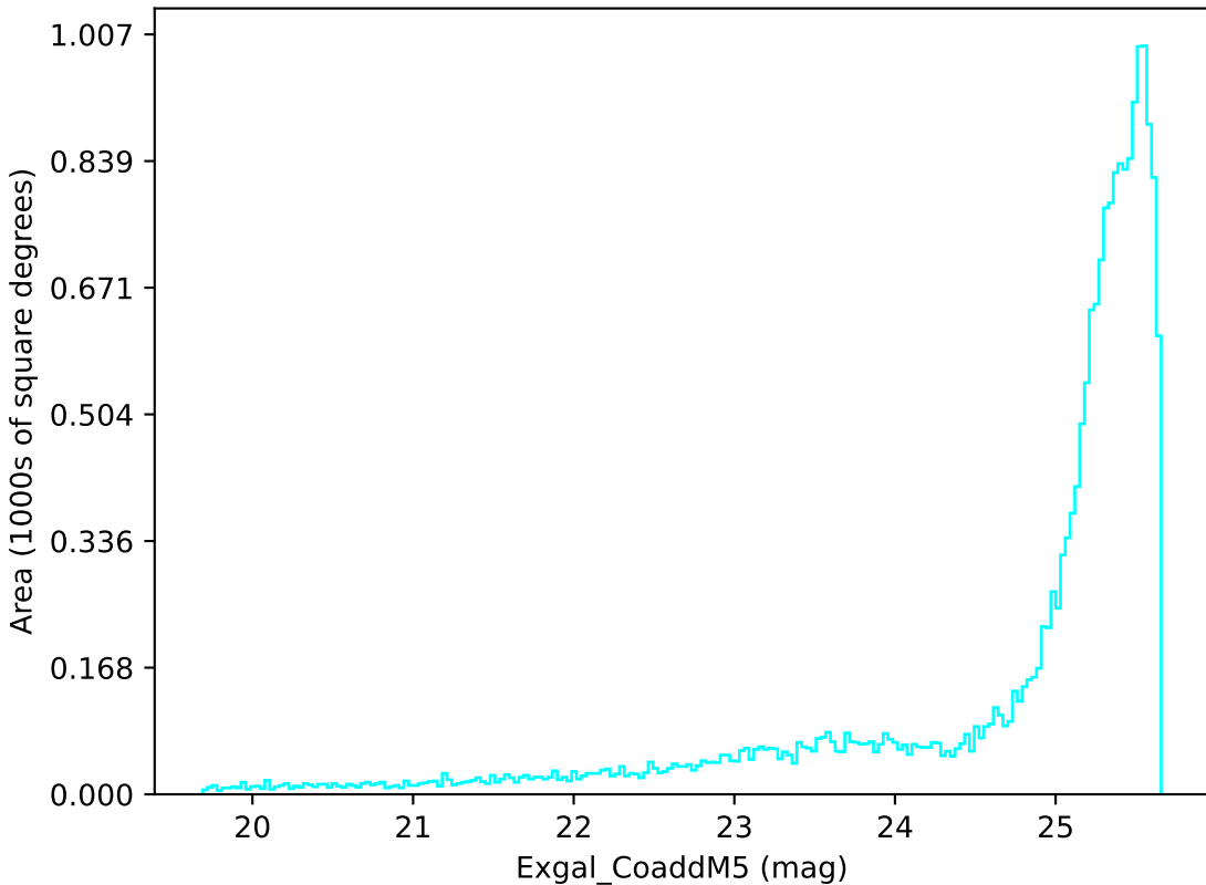
baseline_v3.5_10yrs All sky u band: Exgal_CoaddM5
