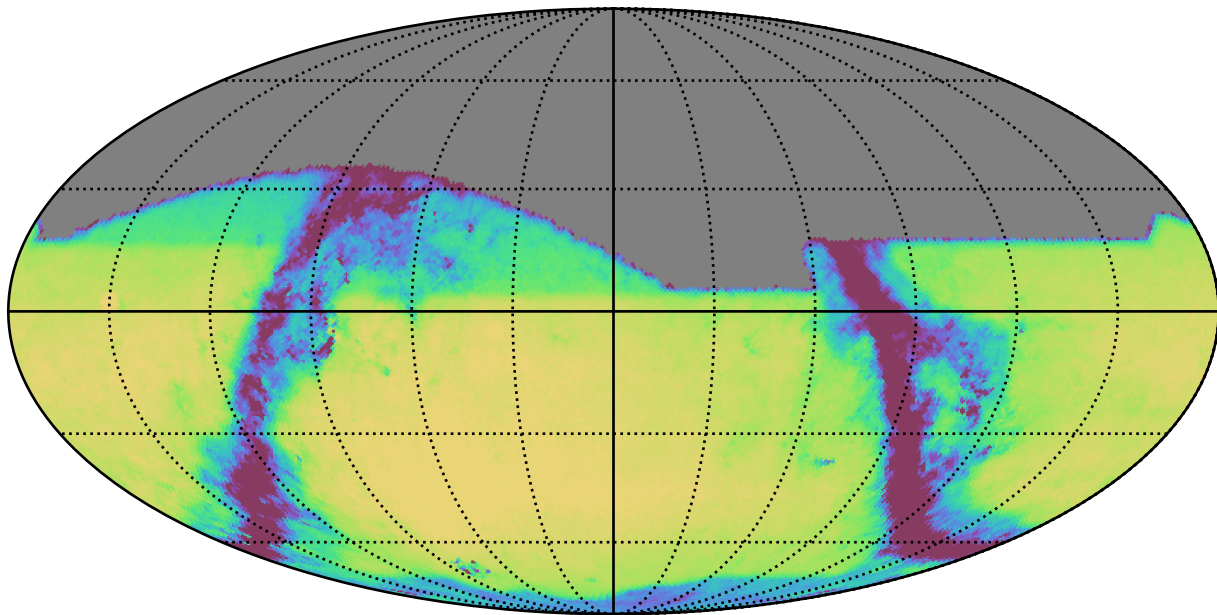
baseline_v3.5_10yrs All sky r band: Exgal_CoaddM5
