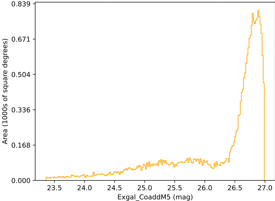
baseline_v3.5_10yrs All sky r band: Exgal_CoaddM5
