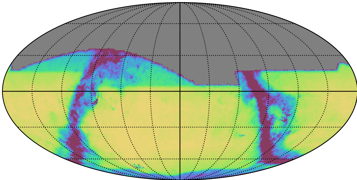
baseline_v3.5_10yrs All sky i band: Exgal_CoaddM5
