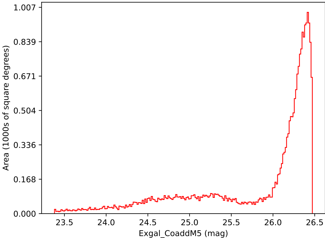
baseline_v3.5_10yrs All sky i band: Exgal_CoaddM5
