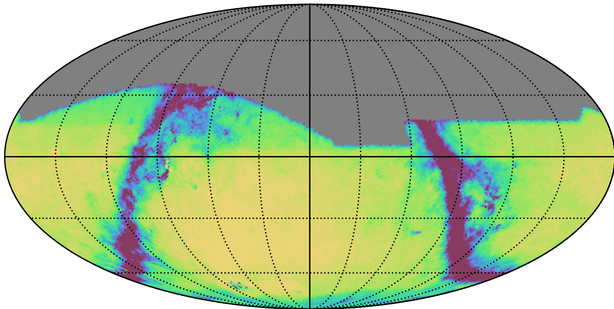
baseline_v3.5_10yrs All sky g band: Exgal_CoaddM5
