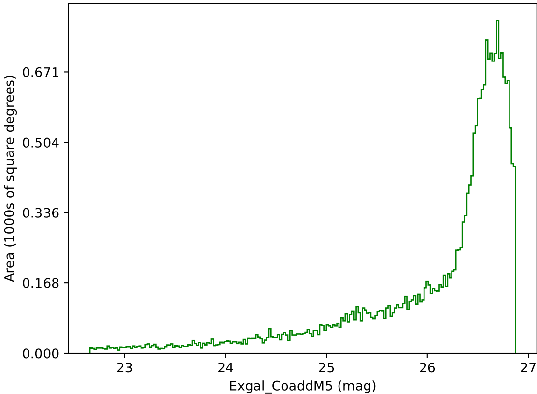
baseline_v3.5_10yrs All sky g band: Exgal_CoaddM5
