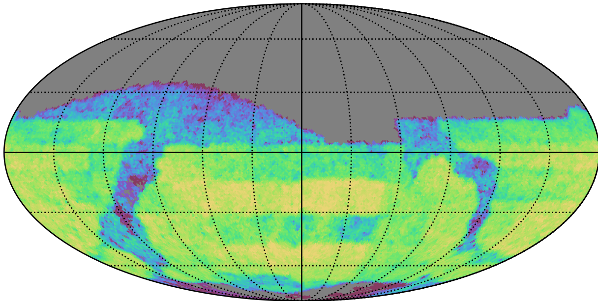
baseline_v3.5_10yrs Yr 3-4 z band: CoaddM5
