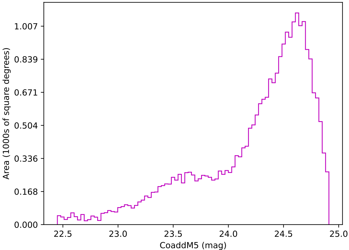
baseline_v3.5_10yrs Yr 3-4 z band: CoaddM5
