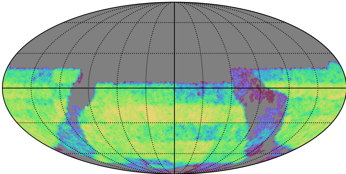
baseline_v3.5_10yrs Yr 3-4 y band: CoaddM5
