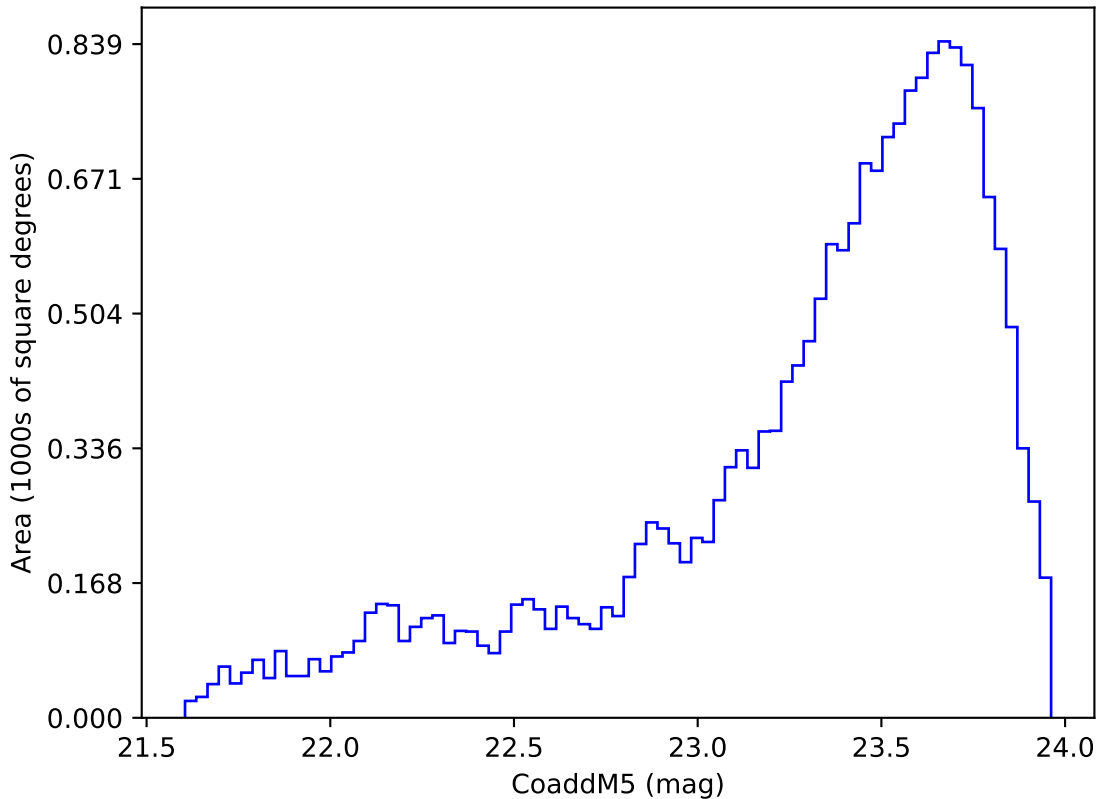
baseline_v3.5_10yrs Yr 3-4 y band: CoaddM5
