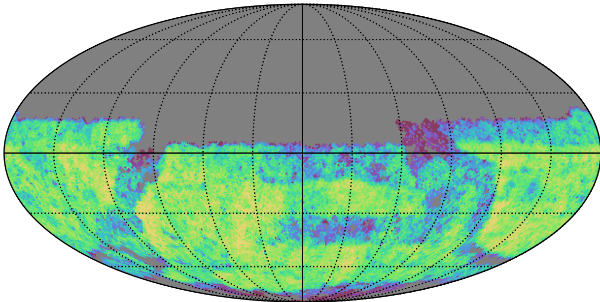
baseline_v3.5_10yrs Yr 3-4 u band: CoaddM5
