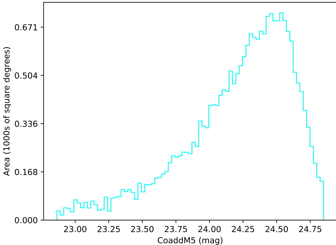
baseline_v3.5_10yrs Yr 3-4 u band: CoaddM5
